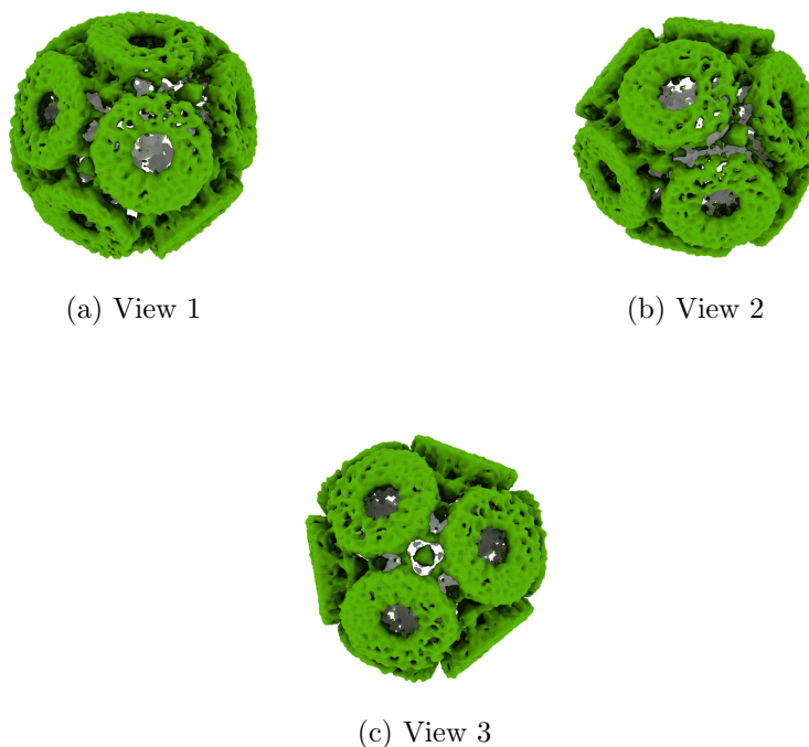
Figure 4: Isosurface at threshold=0.410000. Views generated by ChimeraX at a the following X, Y, Z angles: View 1 (0, -90, -90), View 2 (-90, 0, -90), View 3 (0, 0, 0).
