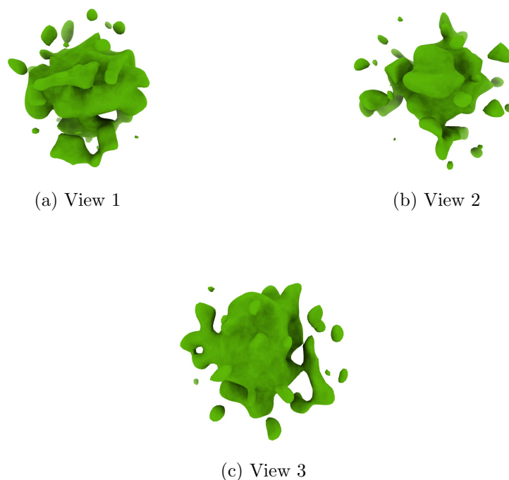
Figure 4: Isosurface at threshold=0.000420. Views generated by ChimeraX at a the following X, Y, Z angles: View 1 (0, -90, -90), View 2 (-90, 0, -90), View 3 (0, 0, 0).
