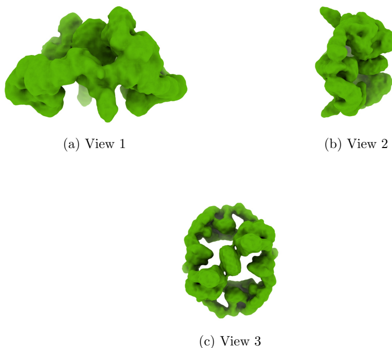
Figure 4: Isosurface at threshold=0.014300. Views generated by ChimeraX at a the following X, Y, Z angles: View 1 (0, -90, -90), View 2 (-90, 0, -90), View 3 (0, 0, 0).
