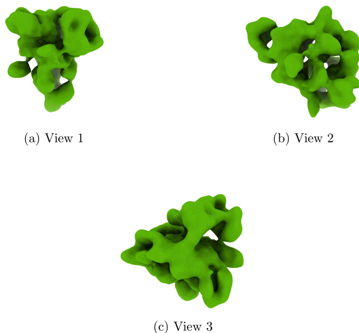
Figure 4: Isosurface at threshold=0.085500. Views generated by ChimeraX at a the following X, Y, Z angles: View 1 (0, -90, -90), View 2 (-90, 0, -90), View 3 (0, 0, 0).
