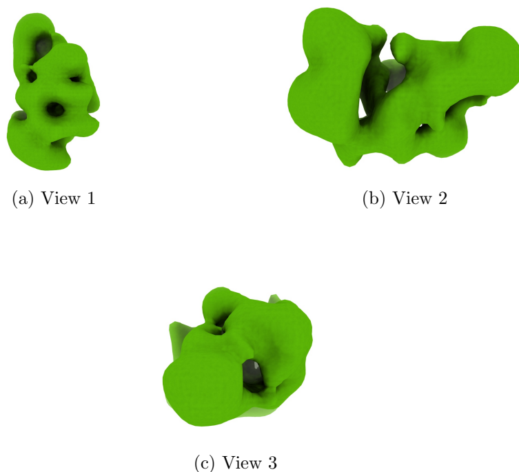
Figure 4: Isosurface at threshold=0.025800. Views generated by ChimeraX at a the following X, Y, Z angles: View 1 (0, -90, -90), View 2 (-90, 0, -90), View 3 (0, 0, 0).
