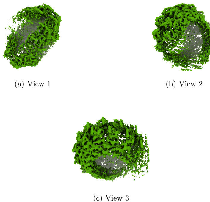
Figure 4: Isosurface at threshold=0.028000. Views generated by ChimeraX at the following X, Y, Z angles: View 1 (0, -90, -90), View 2 (-90, 0, -90), View 3 (0, 0, 0).
