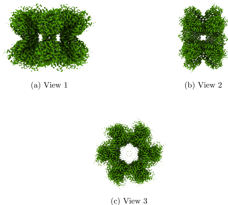
Figure 4: Isosurface at threshold=0.388000. Views generated by ChimeraX at a the following X, Y, Z angles: View 1 (0, -90, -90), View 2 (-90, 0, -90), View 3 (0, 0, 0).
