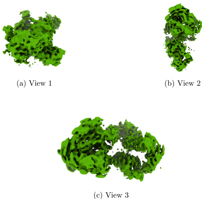
Figure 4: Isosurface at threshold=6.000000. Views generated by ChimeraX at a the following X, Y, Z angles: View 1 (0, -90, -90), View 2 (-90, 0, -90), View 3 (0, 0, 0).
