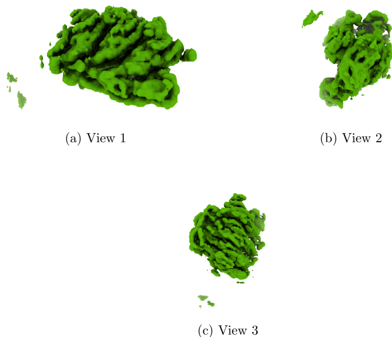
Figure 4: Isosurface at threshold=0.020000. Views generated by ChimeraX at the following X, Y, Z angles: View 1 (0, -90, -90), View 2 (-90, 0, -90), View 3 (0, 0, 0).
