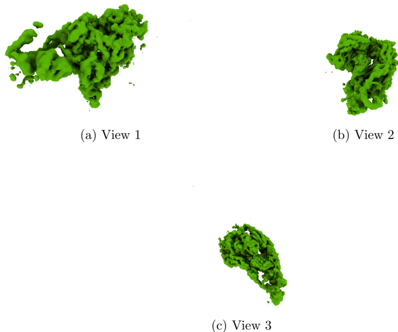
Figure 4: Isosurface at threshold=0.012000. Views generated by ChimeraX at a the following X, Y, Z angles: View 1 (0, -90, -90), View 2 (-90, 0, -90), View 3 (0, 0, 0).
