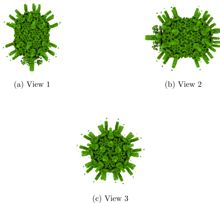
Figure 4: Isosurface at threshold=1.900000. Views generated by ChimeraX at a the following X, Y, Z angles: View 1 (0, -90, -90), View 2 (-90, 0, -90), View 3 (0, 0, 0).
