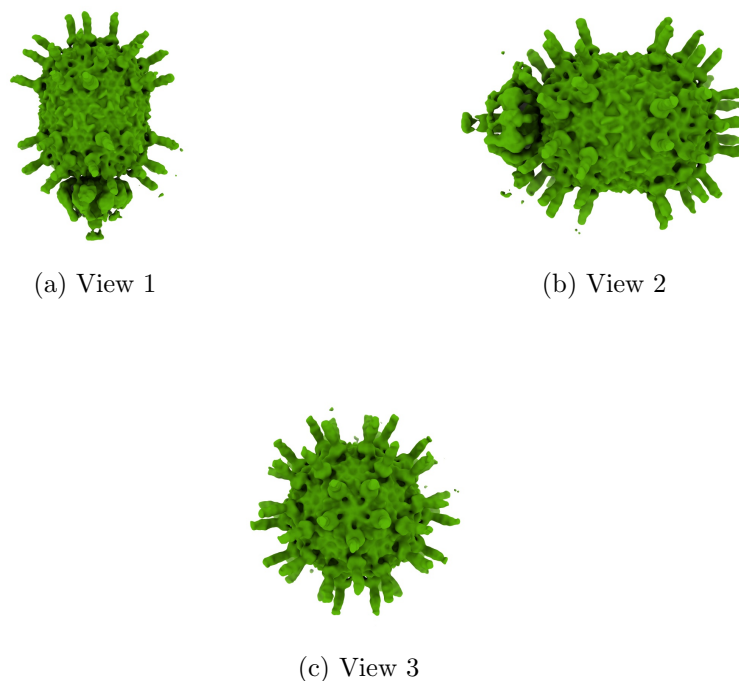
Figure 4: Isosurface at threshold=2.320000. Views generated by ChimeraX at a the following X, Y, Z angles: View 1 (0, -90, -90), View 2 (-90, 0, -90), View 3 (0, 0, 0).
