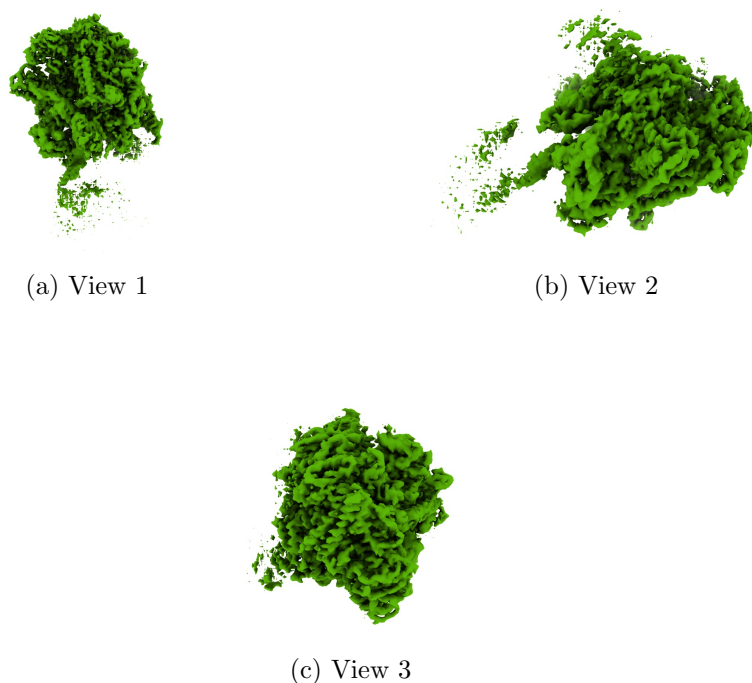
Figure 4: Isosurface at threshold=0.005720. Views generated by ChimeraX at a the following X, Y, Z angles: View 1 (0, -90, -90), View 2 (-90, 0, -90), View 3 (0, 0, 0).
