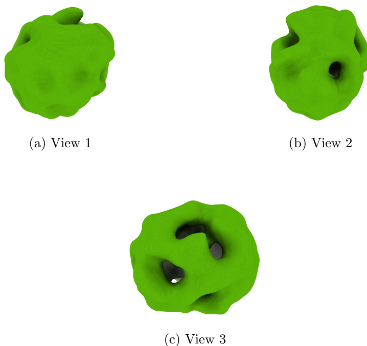
Figure 4: Isosurface at threshold=0.040500. Views generated by ChimeraX at a the following X, Y, Z angles: View 1 (0, -90, -90), View 2 (-90, 0, -90), View 3 (0, 0, 0).
