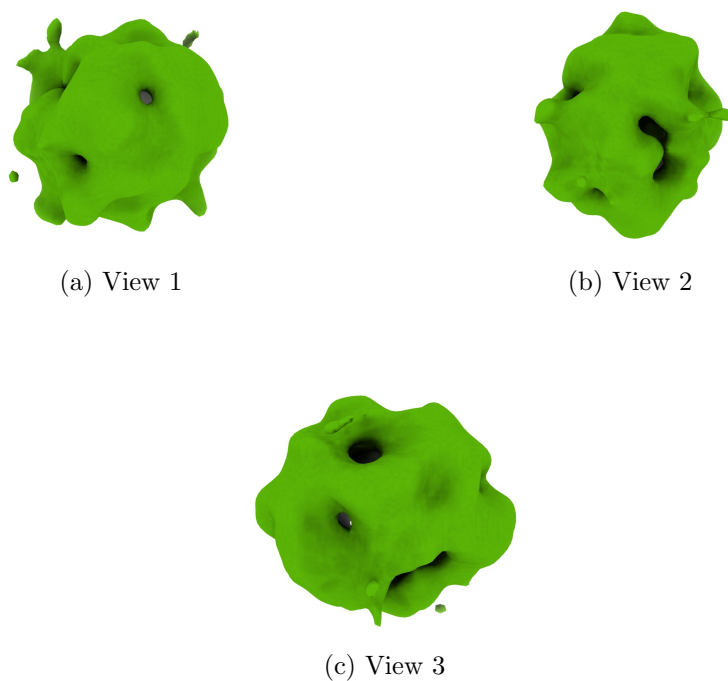
Figure 4: Isosurface at threshold=0.085100. Views generated by ChimeraX at a the following X, Y, Z angles: View 1 (0, -90, -90), View 2 (-90, 0, -90), View 3 (0, 0, 0).
