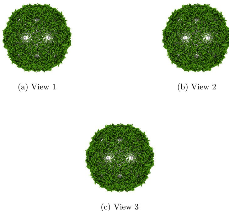
Figure 4: Isosurface at threshold=0.656000. Views generated by ChimeraX at a the following X, Y, Z angles: View 1 (0, -90, -90), View 2 (-90, 0, -90), View 3 (0, 0, 0).
