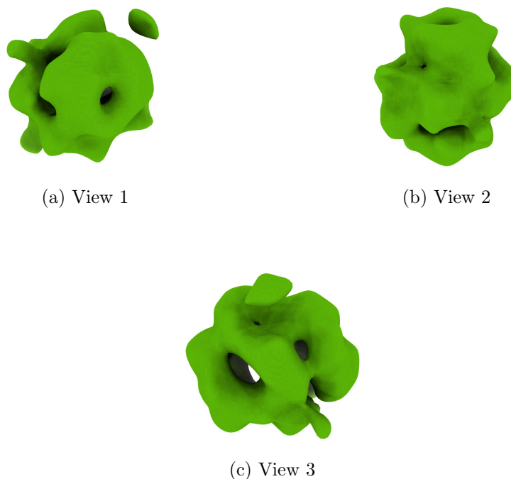
Figure 4: Isosurface at threshold=0.090300. Views generated by ChimeraX at a the following X, Y, Z angles: View 1 (0, -90, -90), View 2 (-90, 0, -90), View 3 (0, 0, 0).
