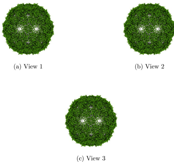
Figure 4: Isosurface at threshold=1.450000. Views generated by ChimeraX at a the following X, Y, Z angles: View 1 (0, -90, -90), View 2 (-90, 0, -90), View 3 (0, 0, 0).
