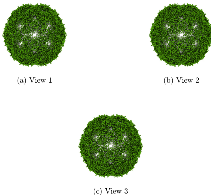
Figure 4: Isosurface at threshold=1.660000. Views generated by ChimeraX at a the following X, Y, Z angles: View 1 (0, -90, -90), View 2 (-90, 0, -90), View 3 (0, 0, 0).
