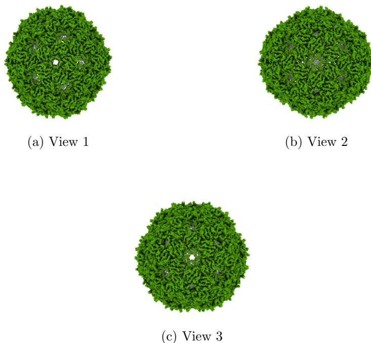
Figure 4: Isosurface at threshold=0.883000. Views generated by ChimeraX at a the following X, Y, Z angles: View 1 (0, -90, -90), View 2 (-90, 0, -90), View 3 (0, 0, 0).
