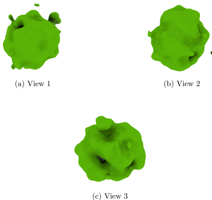
Figure 4: Isosurface at threshold=0.041500. Views generated by ChimeraX at a the following X, Y, Z angles: View 1 (0, -90, -90), View 2 (-90, 0, -90), View 3 (0, 0, 0).
