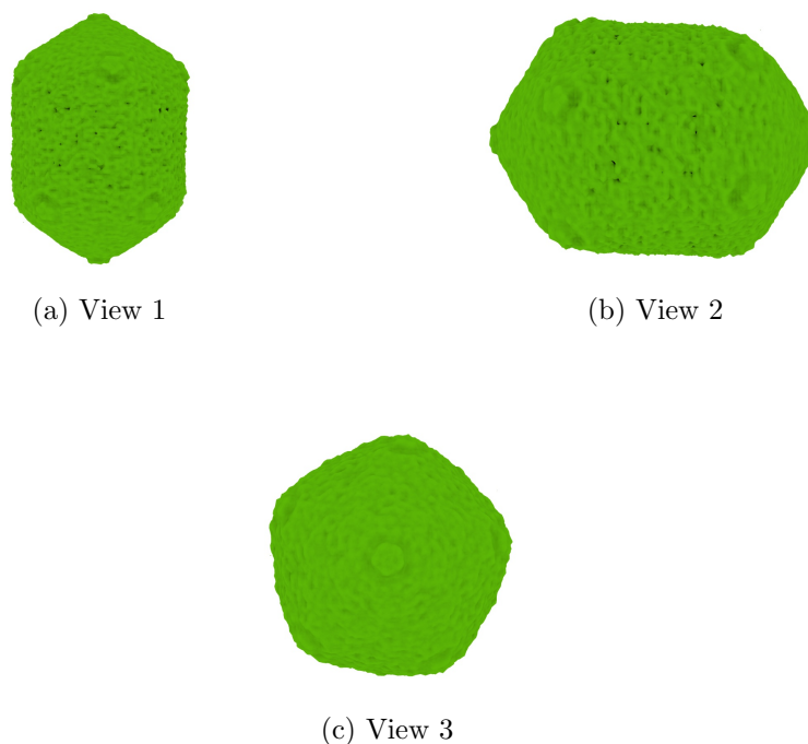
Figure 4: Isosurface at threshold=0.332000. Views generated by ChimeraX at a the following X, Y, Z angles: View 1 (0, -90, -90), View 2 (-90, 0, -90), View 3 (0, 0, 0).
