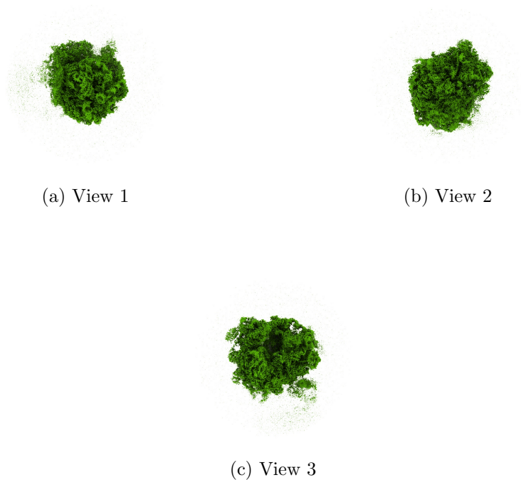
Figure 4: Isosurface at threshold=0.016200. Views generated by ChimeraX at a the following X, Y, Z angles: View 1 (0, -90, -90), View 2 (-90, 0, -90), View 3 (0, 0, 0).
