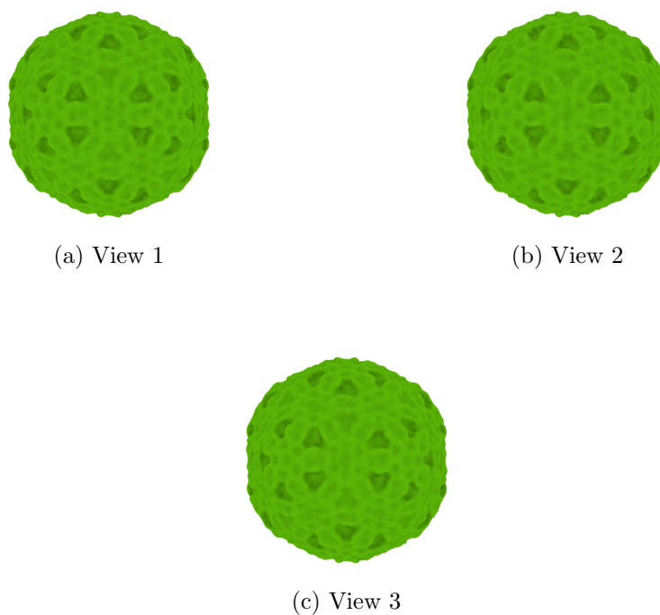
Figure 4: Isosurface at threshold=4.660000. Views generated by ChimeraX at a the following X, Y, Z angles: View 1 (0, -90, -90), View 2 (-90, 0, -90), View 3 (0, 0, 0).
