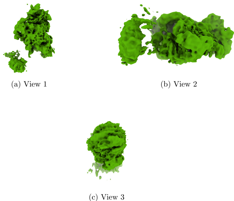
Figure 4: Isosurface at threshold=0.237000. Views generated by ChimeraX at a the following X, Y, Z angles: View 1 (0, -90, -90), View 2 (-90, 0, -90), View 3 (0, 0, 0).
