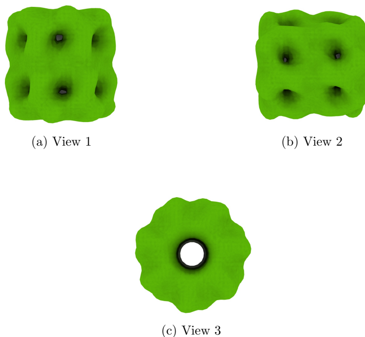
Figure 4: Isosurface at threshold=0.006360. Views generated by ChimeraX at a the following X, Y, Z angles: View 1 (0, -90, -90), View 2 (-90, 0, -90), View 3 (0, 0, 0).
