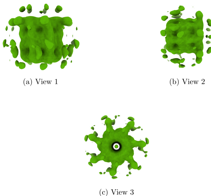
Figure 4: Isosurface at threshold=0.001850. Views generated by ChimeraX at a the following X, Y, Z angles: View 1 (0, -90, -90), View 2 (-90, 0, -90), View 3 (0, 0, 0).
