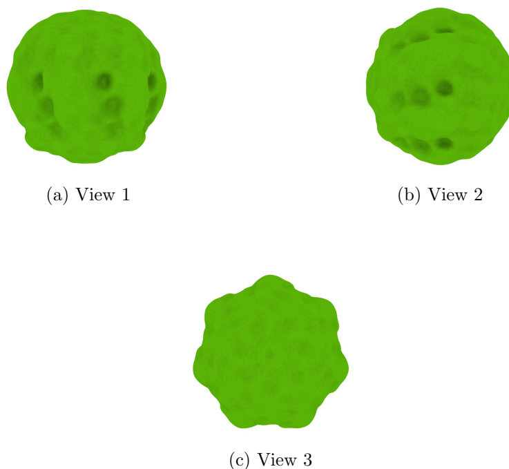
Figure 4: Isosurface at threshold=2.270000. Views generated by ChimeraX at a the following X, Y, Z angles: View 1 (0, -90, -90), View 2 (-90, 0, -90), View 3 (0, 0, 0).
