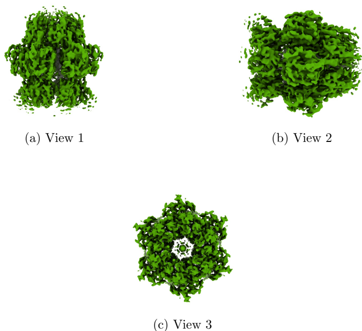
Figure 4: Isosurface at threshold=0.010900. Views generated by ChimeraX at a the following X, Y, Z angles: View 1 (0, -90, -90), View 2 (-90, 0, -90), View 3 (0, 0, 0).
