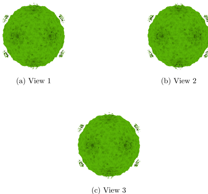
Figure 4: Isosurface at threshold=10400.000000. Views generated by ChimeraX at the following X, Y, Z angles: View 1 (0, -90, -90), View 2 (-90, 0, -90), View 3 (0, 0, 0).
