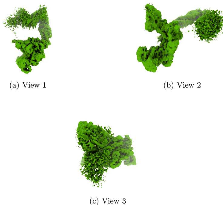
Figure 4: Isosurface at threshold=0.010500. Views generated by ChimeraX at a the following X, Y, Z angles: View 1 (0, -90, -90), View 2 (-90, 0, -90), View 3 (0, 0, 0).
