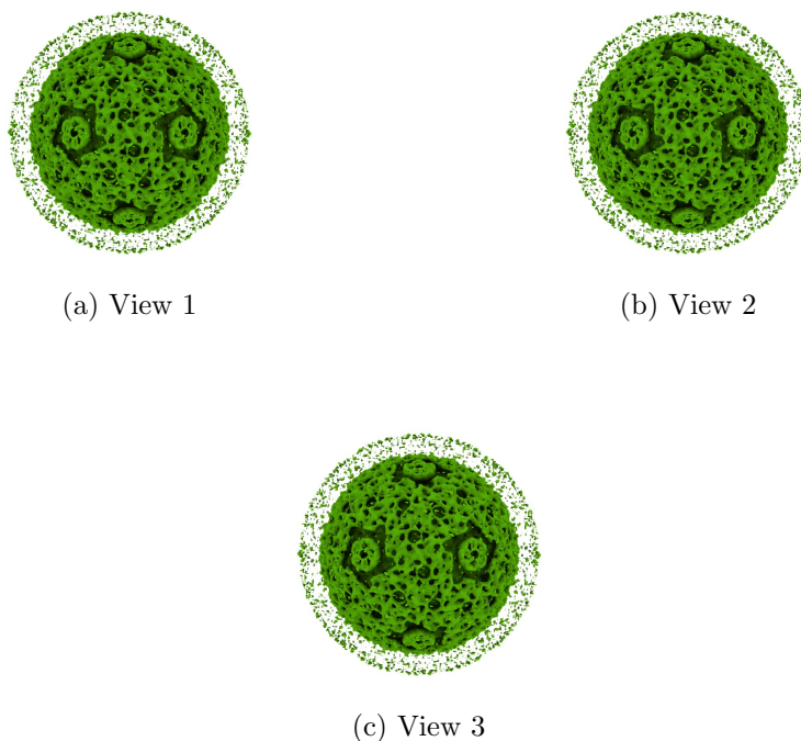
Figure 4: Isosurface at threshold=1700.000000. Views generated by ChimeraX at the following X, Y, Z angles: View 1 (0, -90, -90), View 2 (-90, 0, -90), View 3 (0, 0, 0).
