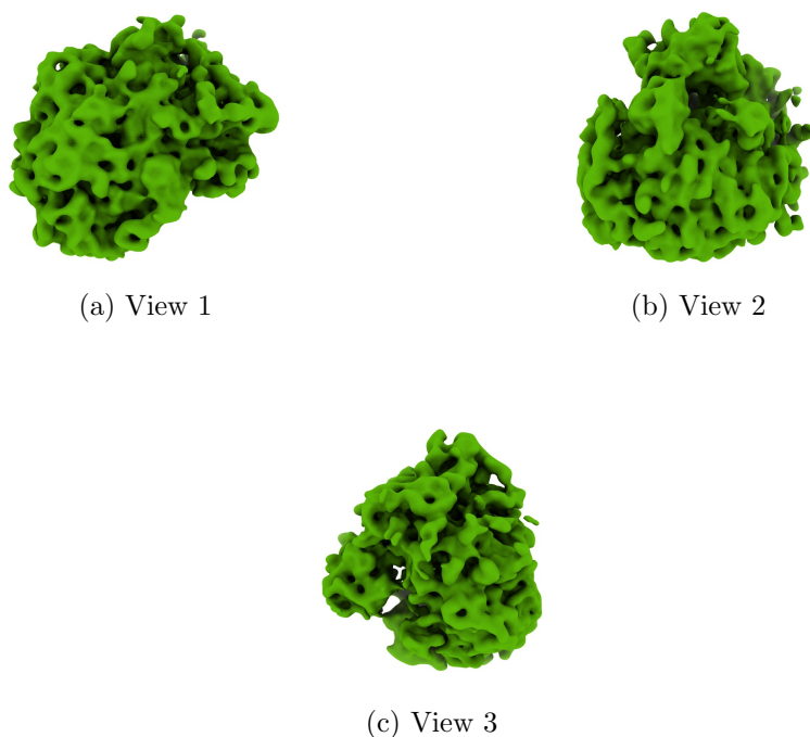
Figure 4: Isosurface at threshold=74.300000. Views generated by ChimeraX at a the following X, Y, Z angles: View 1 (0, -90, -90), View 2 (-90, 0, -90), View 3 (0, 0, 0).
