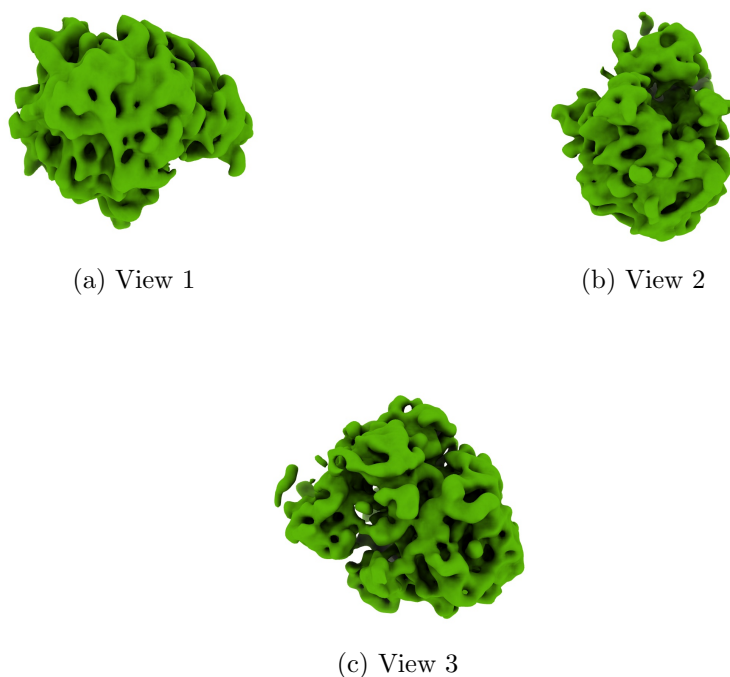
Figure 4: Isosurface at threshold=73.200000. Views generated by ChimeraX at a the following X, Y, Z angles: View 1 (0, -90, -90), View 2 (-90, 0, -90), View 3 (0, 0, 0).
