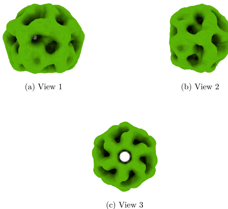
Figure 4: Isosurface at threshold=0.305000. Views generated by ChimeraX at a the following X, Y, Z angles: View 1 (0, -90, -90), View 2 (-90, 0, -90), View 3 (0, 0, 0).
