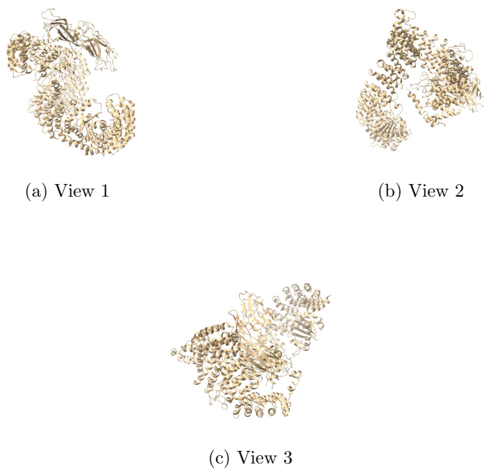
Figure 10: Input atomic model Views generated by ChimeraX at a the following X, Y, Z angles: View 1 (0, -90, -90), View 2 (-90, 0, -90), View 3 (0, 0, 0).
