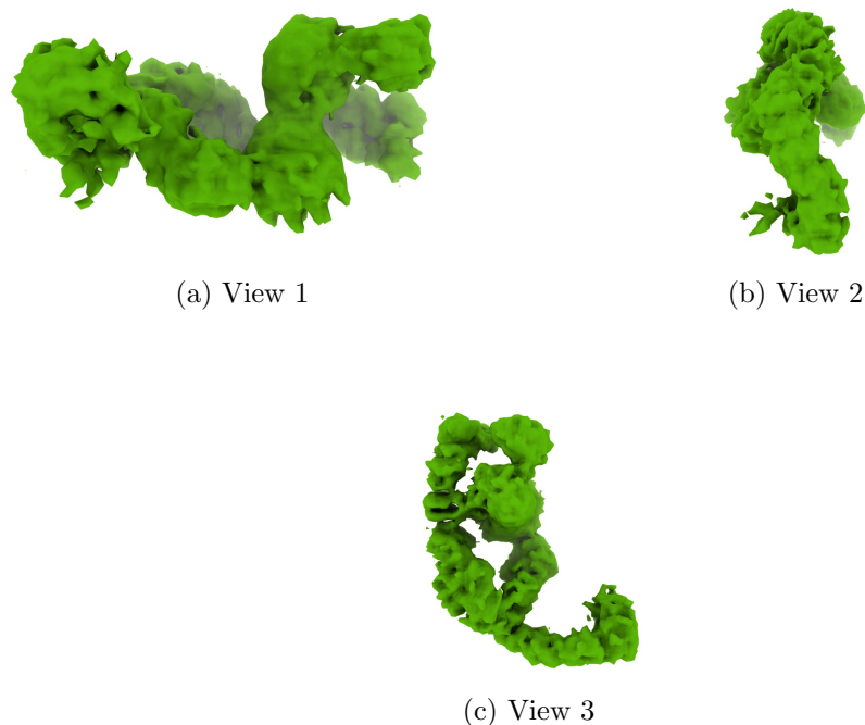
Figure 4: Isosurface at threshold=0.070000. Views generated by ChimeraX at a the following X, Y, Z angles: View 1 (0, -90, -90), View 2 (-90, 0, -90), View 3 (0, 0, 0).
