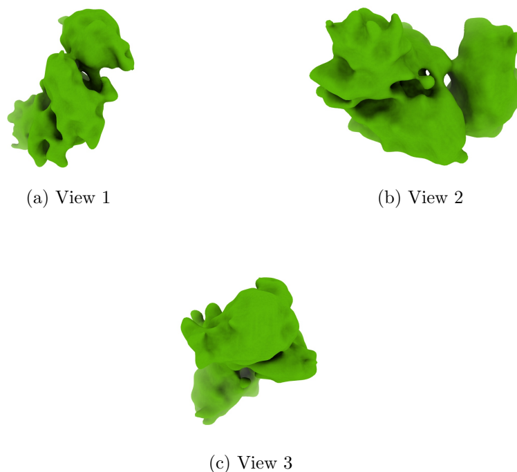
Figure 4: Isosurface at threshold=10.600000. Views generated by ChimeraX at a the following X, Y, Z angles: View 1 (0, -90, -90), View 2 (-90, 0, -90), View 3 (0, 0, 0).
