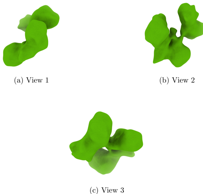
Figure 4: Isosurface at threshold=9.880000. Views generated by ChimeraX at a the following X, Y, Z angles: View 1 (0, -90, -90), View 2 (-90, 0, -90), View 3 (0, 0, 0).
