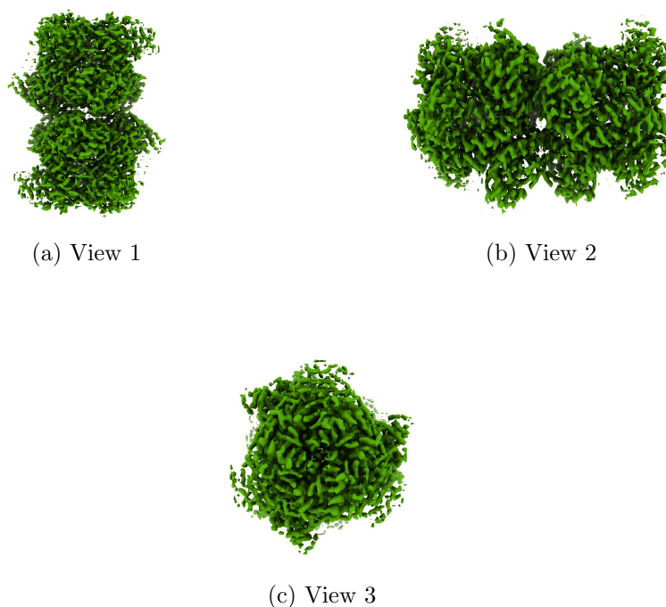
Figure 4: Isosurface at threshold=0.018300. Views generated by ChimeraX at a the following X, Y, Z angles: View 1 (0, -90, -90), View 2 (-90, 0, -90), View 3 (0, 0, 0).
