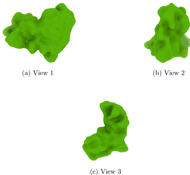
Figure 4: Isosurface at threshold=3.720000. Views generated by ChimeraX at a the following X, Y, Z angles: View 1 (0, -90, -90), View 2 (-90, 0, -90), View 3 (0, 0, 0).
