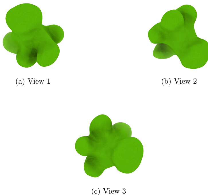
Figure 4: Isosurface at threshold=0.028400. Views generated by ChimeraX at a the following X, Y, Z angles: View 1 (0, -90, -90), View 2 (-90, 0, -90), View 3 (0, 0, 0).
