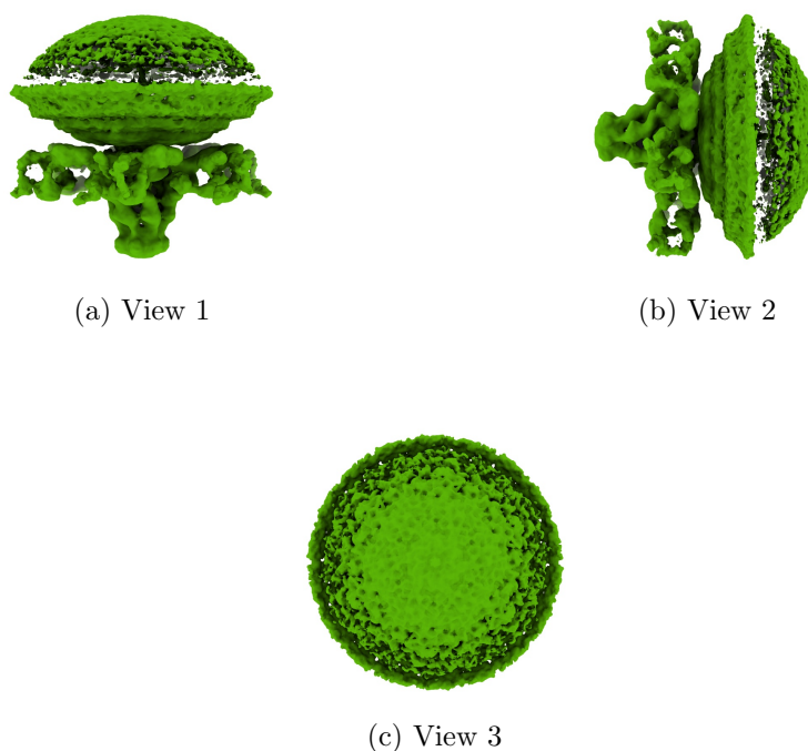
Figure 4: Isosurface at threshold=1.920000. Views generated by ChimeraX at a the following X, Y, Z angles: View 1 (0, -90, -90), View 2 (-90, 0, -90), View 3 (0, 0, 0).
