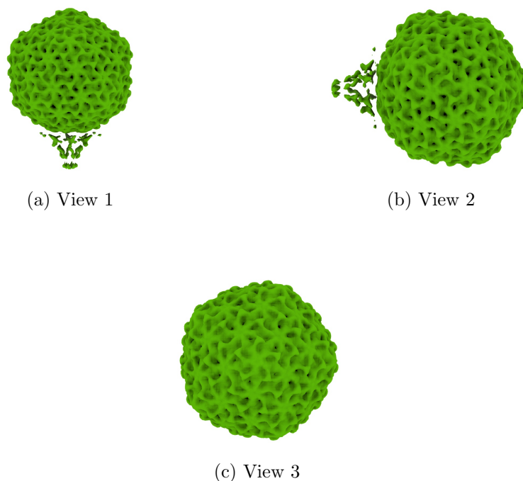
Figure 4: Isosurface at threshold=3.060000. Views generated by ChimeraX at a the following X, Y, Z angles: View 1 (0, -90, -90), View 2 (-90, 0, -90), View 3 (0, 0, 0).
