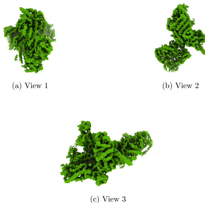
Figure 4: Isosurface at threshold=0.014900. Views generated by ChimeraX at a the following X, Y, Z angles: View 1 (0, -90, -90), View 2 (-90, 0, -90), View 3 (0, 0, 0).
