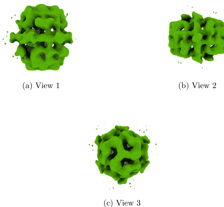
Figure 4: Isosurface at threshold=0.093100. Views generated by ChimeraX at a the following X, Y, Z angles: View 1 (0, -90, -90), View 2 (-90, 0, -90), View 3 (0, 0, 0).
