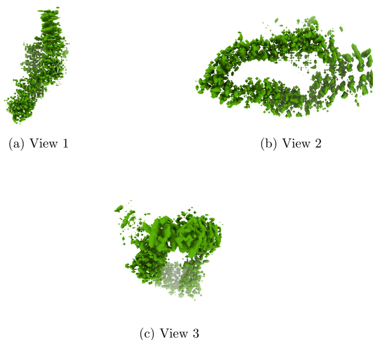
Figure 4: Isosurface at threshold=0.230000. Views generated by ChimeraX at the following X, Y, Z angles: View 1 (0, -90, -90), View 2 (-90, 0, -90), View 3 (0, 0, 0).
