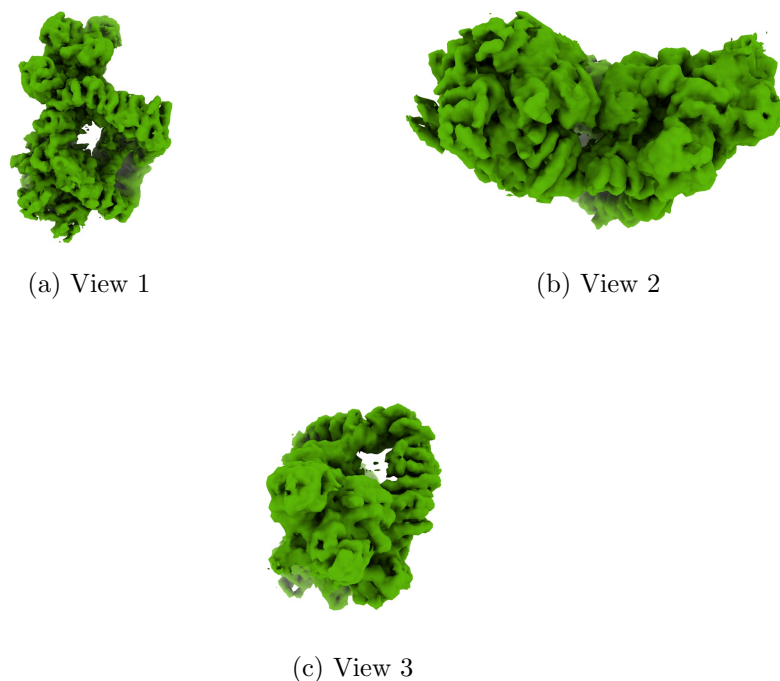
Figure 4: Isosurface at threshold=0.306000. Views generated by ChimeraX at a the following X, Y, Z angles: View 1 (0, -90, -90), View 2 (-90, 0, -90), View 3 (0, 0, 0).
