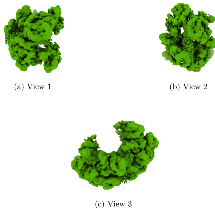
Figure 4: Isosurface at threshold=0.005380. Views generated by ChimeraX at a the following X, Y, Z angles: View 1 (0, -90, -90), View 2 (-90, 0, -90), View 3 (0, 0, 0).
