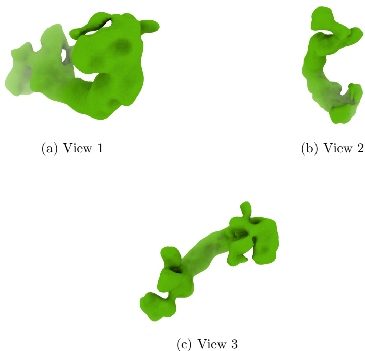
Figure 4: Isosurface at threshold=0.030300. Views generated by ChimeraX at a the following X, Y, Z angles: View 1 (0, -90, -90), View 2 (-90, 0, -90), View 3 (0, 0, 0).
